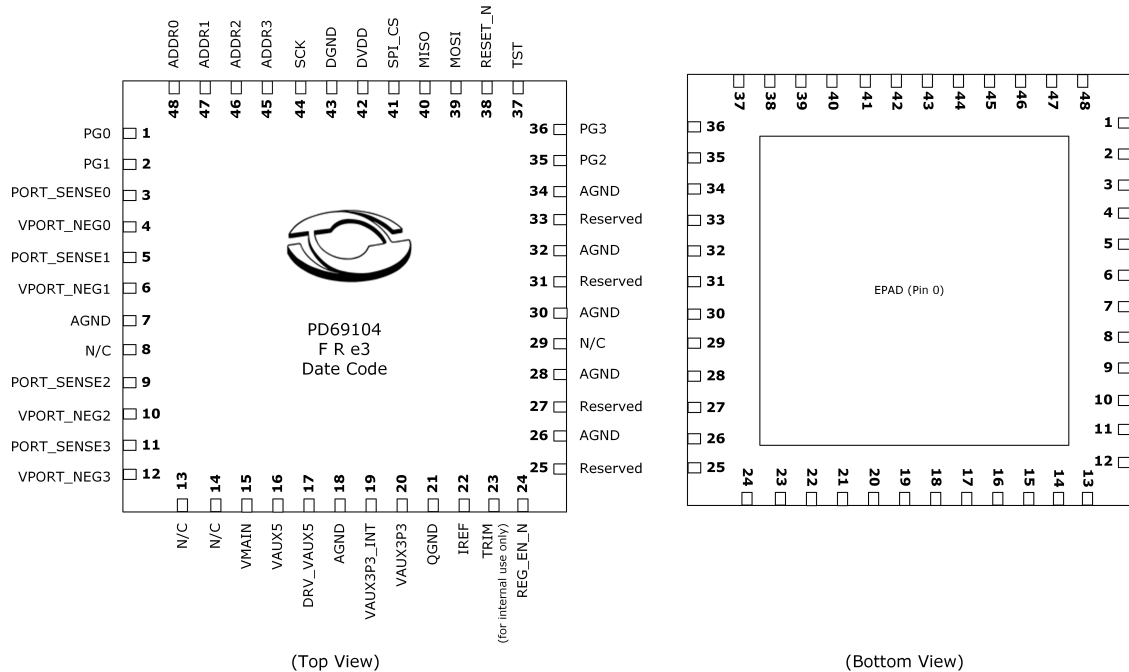
Figure 5 • PD69104 Pinout
