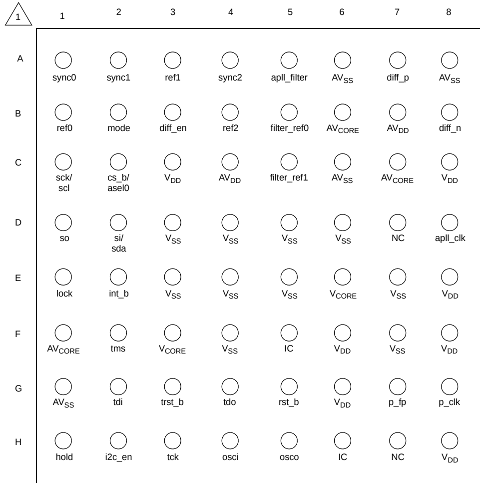
TOP VIEW
