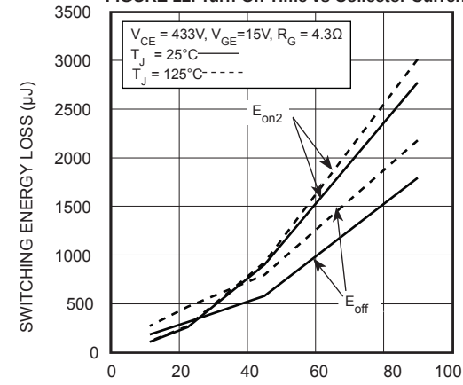
FIGURE 14. Energy Loss vs Collector Current
