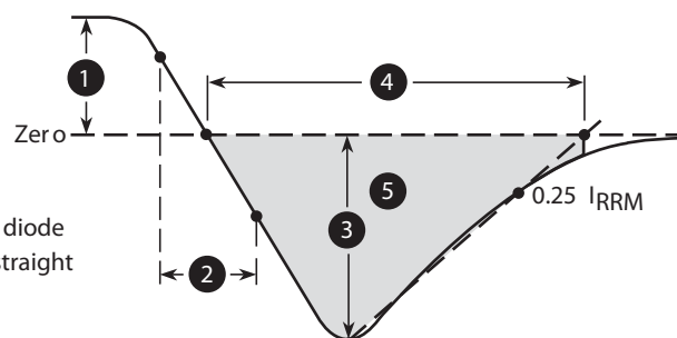
Figure 10. Diode Reverse Recovery and Definitions
