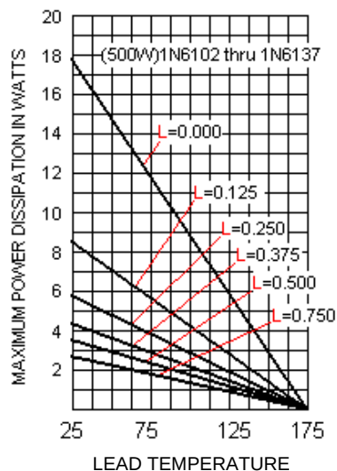
FIGURE 4 MAXIMUM POWER vs. LEAD TEMPERATURE
