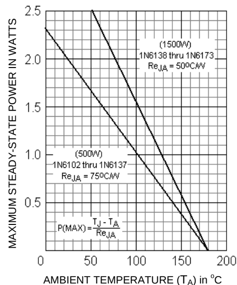
FIGURE 5 STEADY-STATE DERATING CURVE FOR FREE-AIR MOUNTING (For PC boards where thermal resistance from mounting point to ambient is sufficiently controlled where T_{OP} or T_{J(MAX)} rating is not exceeded)
