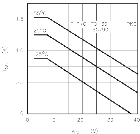
Figure 4 – Short-circuit Current vs. V_{IN}
