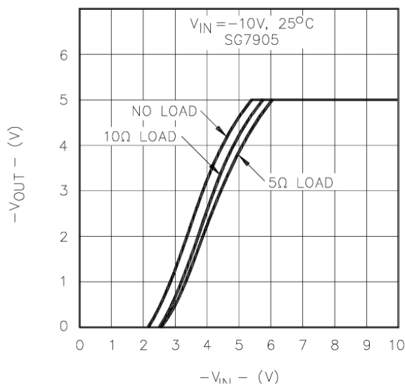
Figure 7 – Dropout Characteristics
