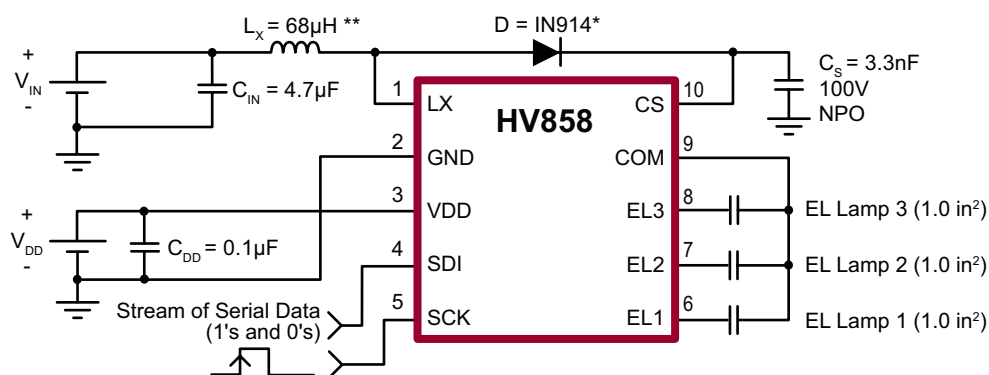
Fig. 1: Test Circuit
