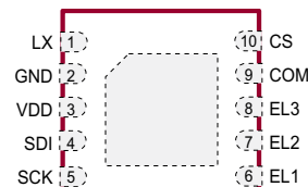
10-Lead DFN (K7) (top view)
