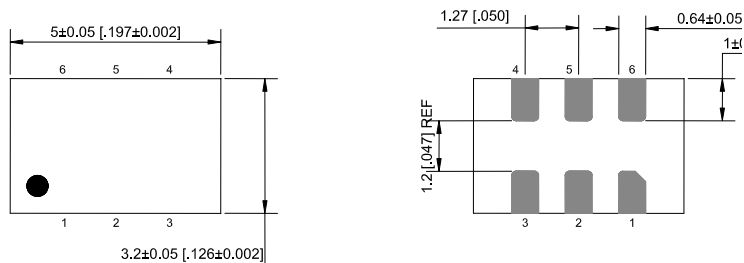
External Dimensions
