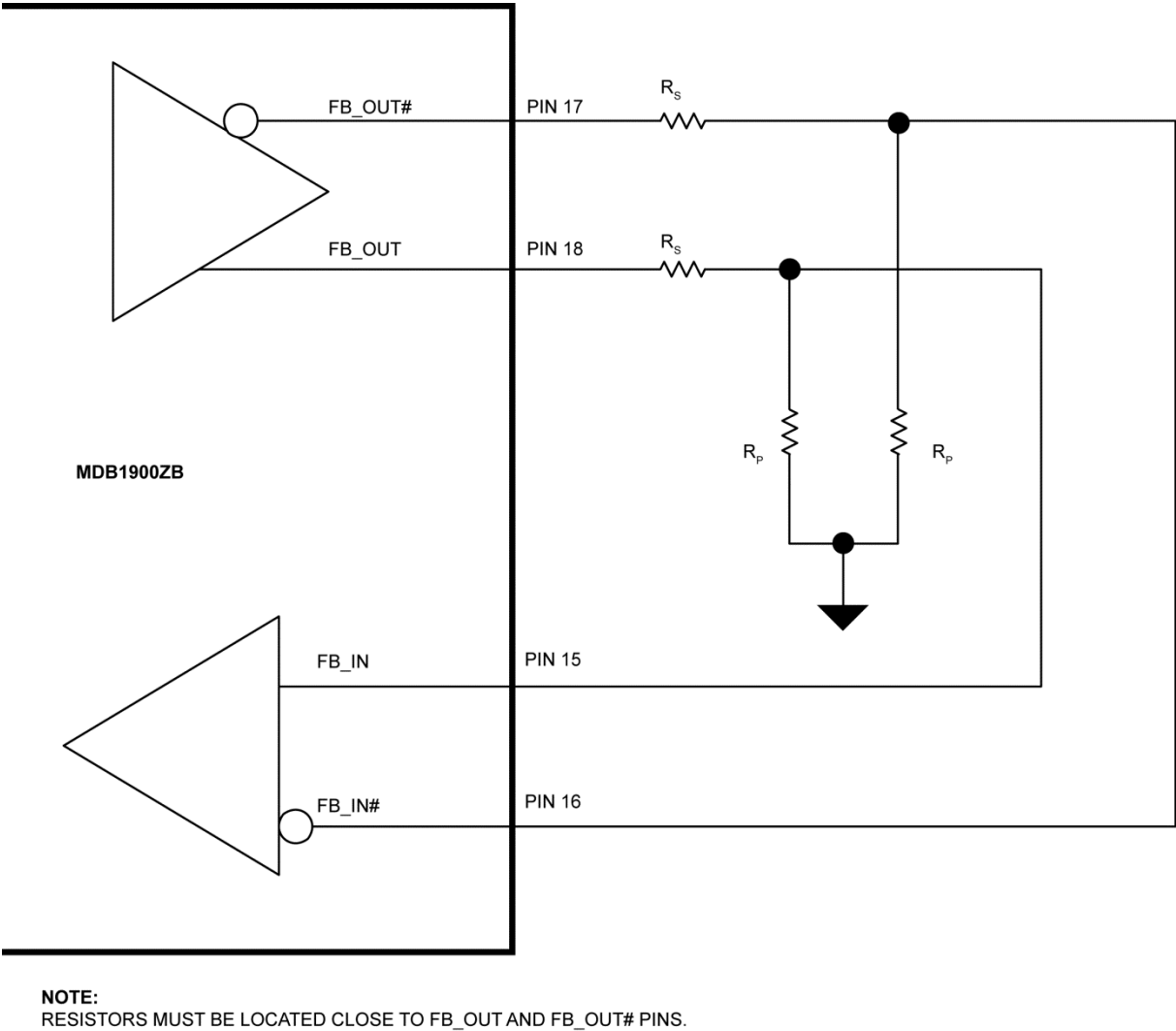
Figure 1. External Feedback
