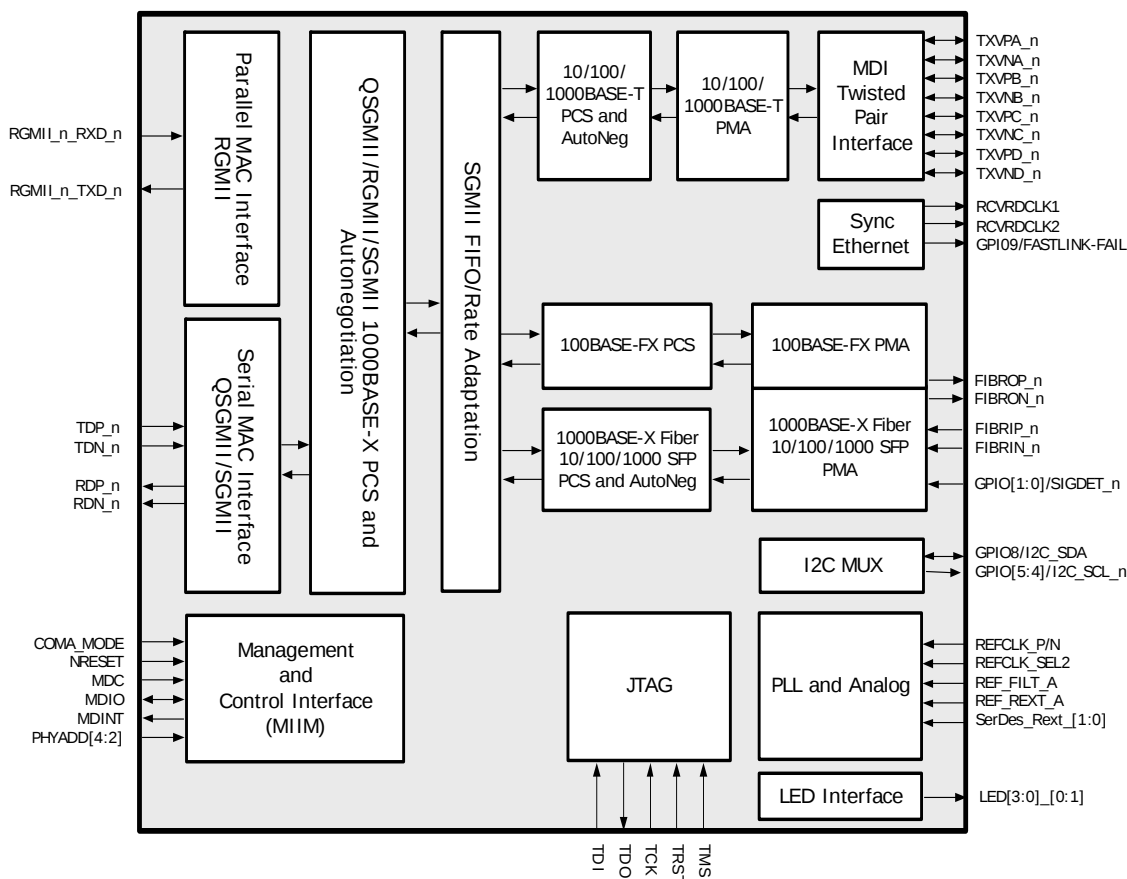
Figure 4 • Block Diagram
