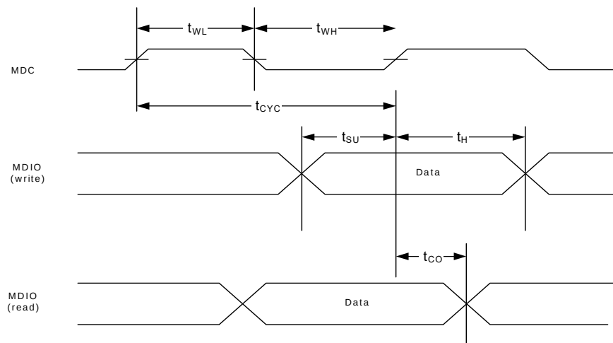
Figure 53 • Serial Management Interface Timing
