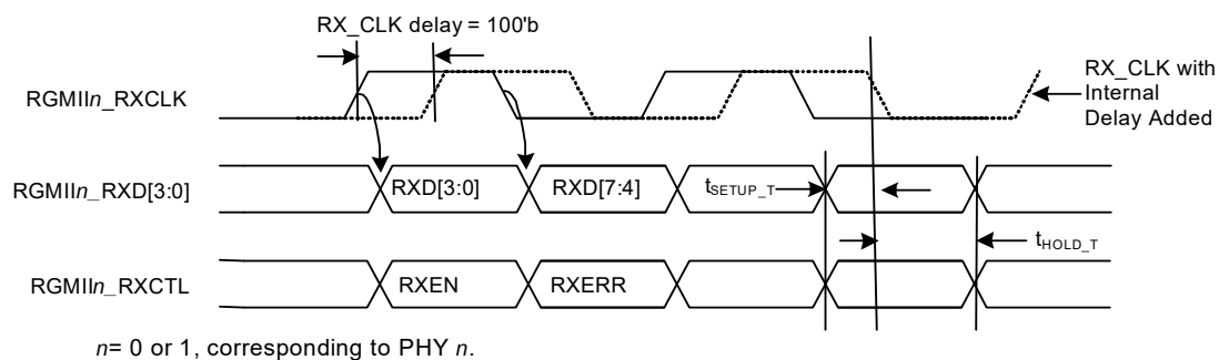
Figure 52 • Compensated Output RGMII Timing
