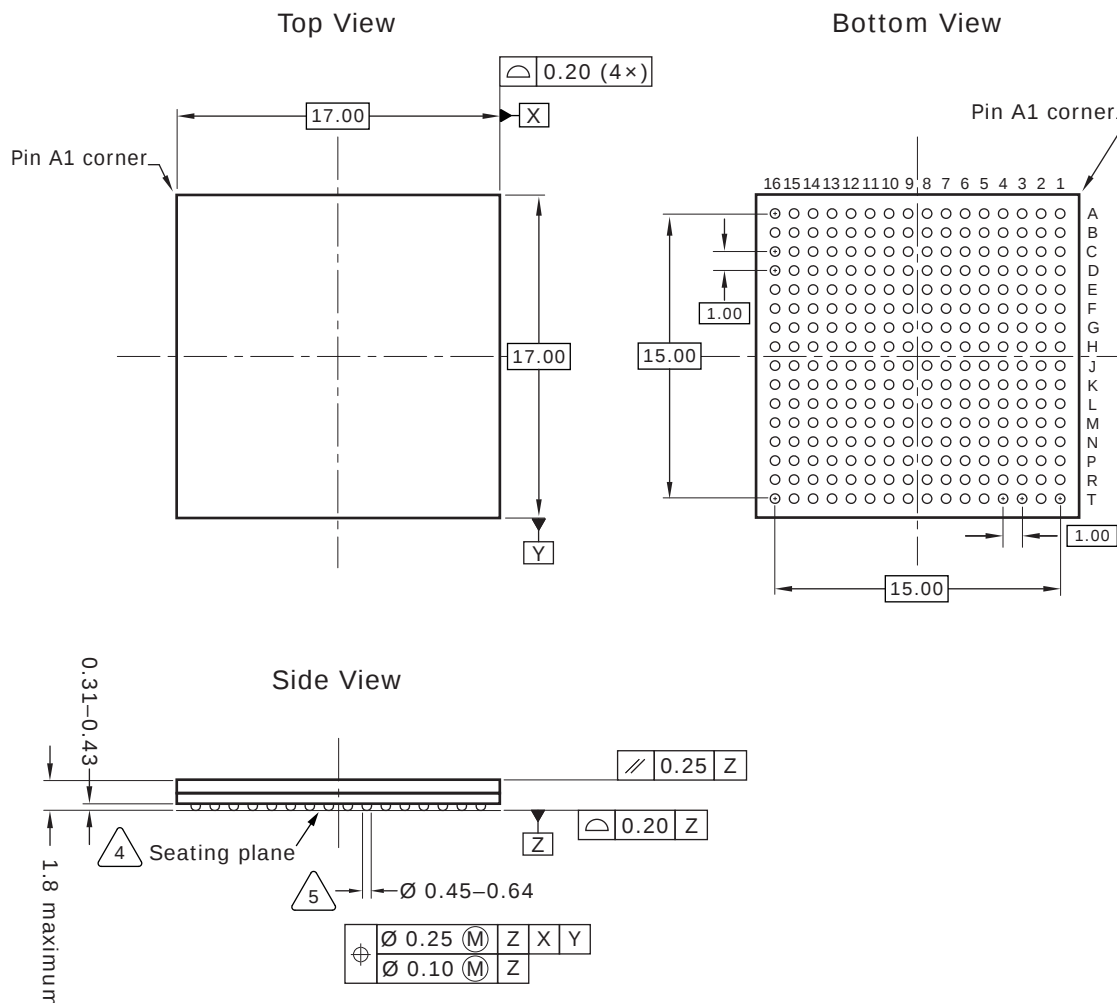
Figure 56 • Package Drawing
