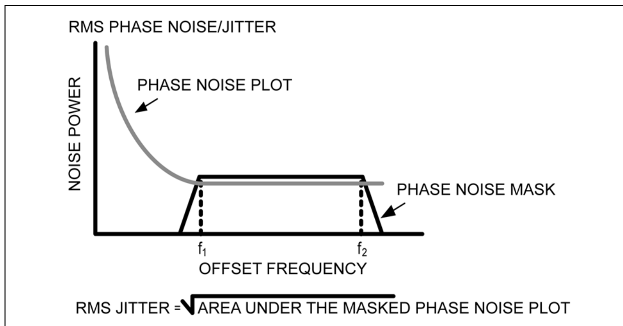
FIGURE 6-1: RMS Phase/Noise/Jitter.
