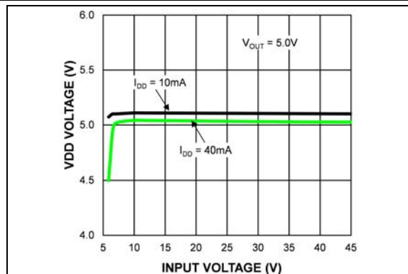
FIGURE 2-4: V_{DD} Voltage vs. Input Voltage.
