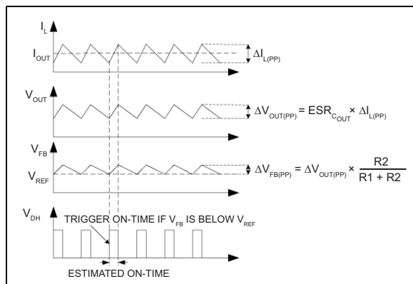
FIGURE 4-2: MIC28513 Control Loop Timing.
