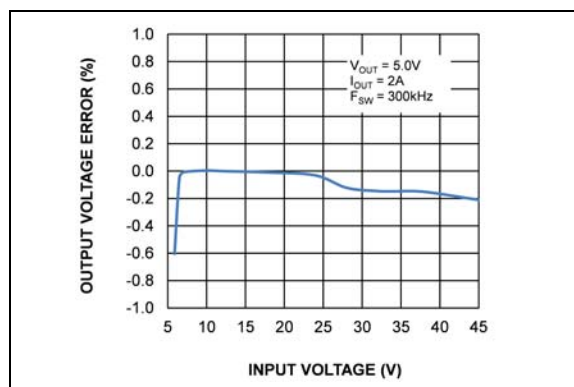
FIGURE 2-6: Line Regulation ( V_{OUT} Error vs. V_{IN} ).
