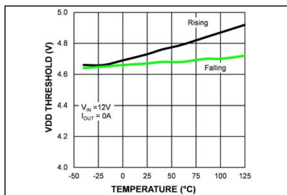
FIGURE 2-5: V_{DD} UVLO Threshold vs. Temperature (MIC28513-1).
