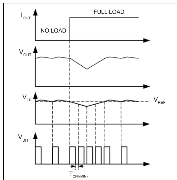
FIGURE 4-3: MIC28513 Load Transient Response.
