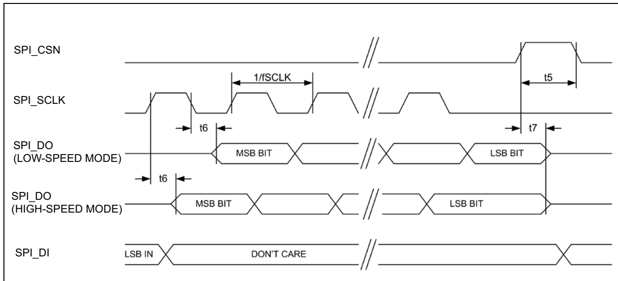
FIGURE 7-9: SPI INTERFACE DATA OUTPUT TIMING
