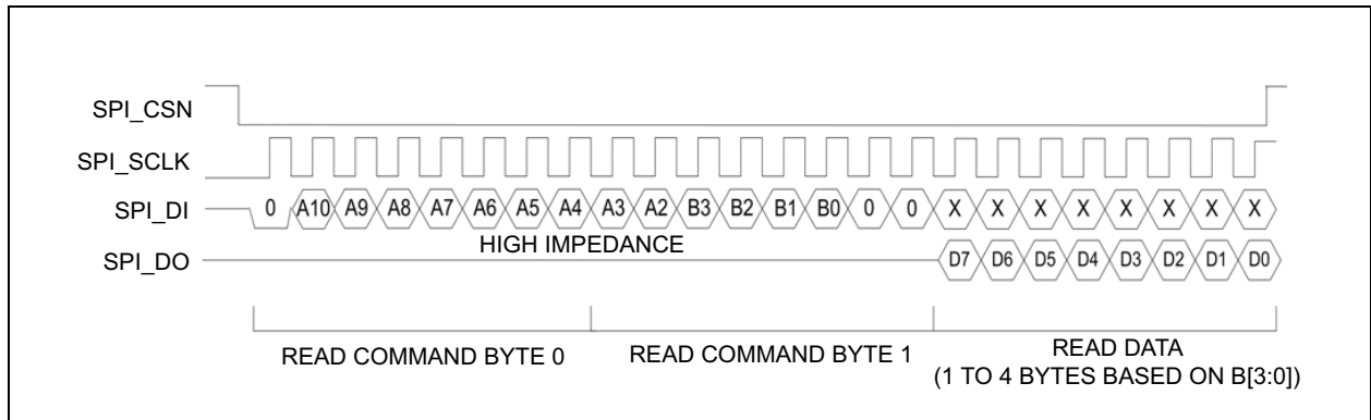
FIGURE 3-19: SPI REGISTER READ OPERATION – HIGH-SPEED MODE
