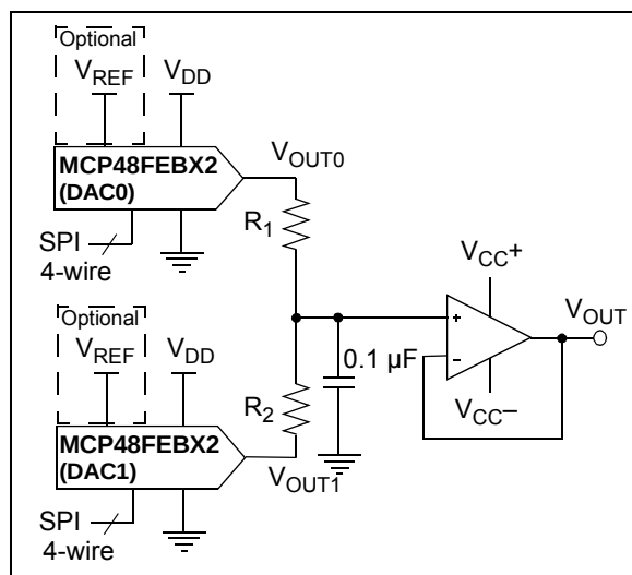
FIGURE 8-6: Simple Double-Precision DAC using MCP48FEBX2.
