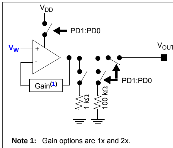
FIGURE 5-10: V_{OUT} Power-Down Block Diagram.
