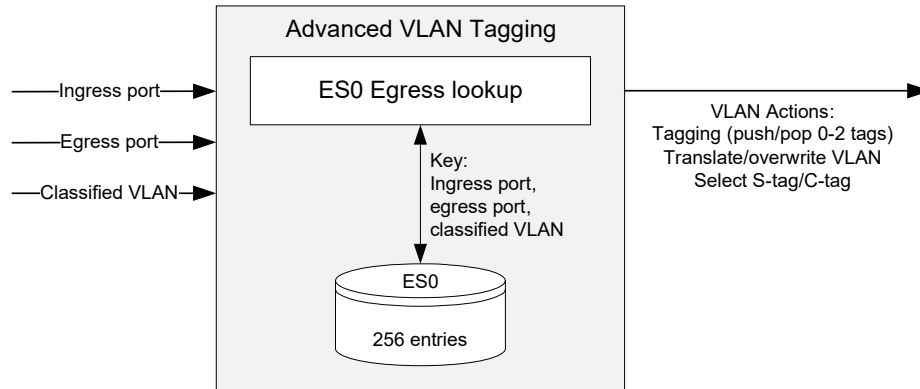
Figure 5 • Advanced VLAN Tagging
