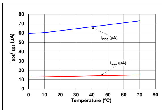
FIGURE 4-4: I_{DDQ}/I_{SS} vs. Temperature.
