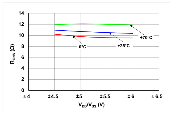
FIGURE 4-1: R_{ONS} at 5 mA vs. V_{DD}/V_{SS} .
