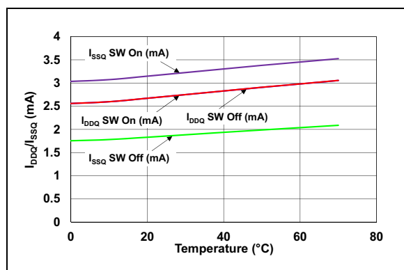
FIGURE 4-3: I_{DDQ}/I_{SSQ} vs. Temperature.
