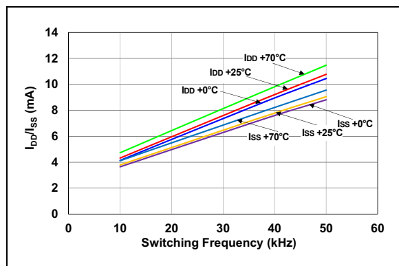
FIGURE 4-2: I_{DDQ}/I_{SS} vs. Switching Frequency.
