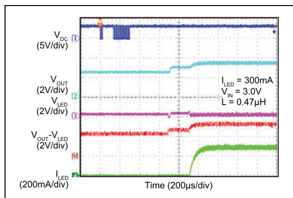
FIGURE 2-15: Torch Mode Turn-On Sequence (Boost Mode).
