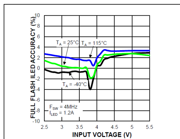
FIGURE 2-12: Full Flash ILED Accuracy vs. Input Voltage.
