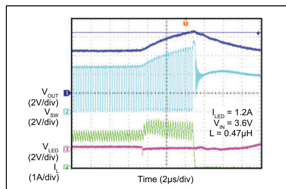
FIGURE 2-24: V_{OUT} Overvoltage Protection (Overvoltage after Start-up).
