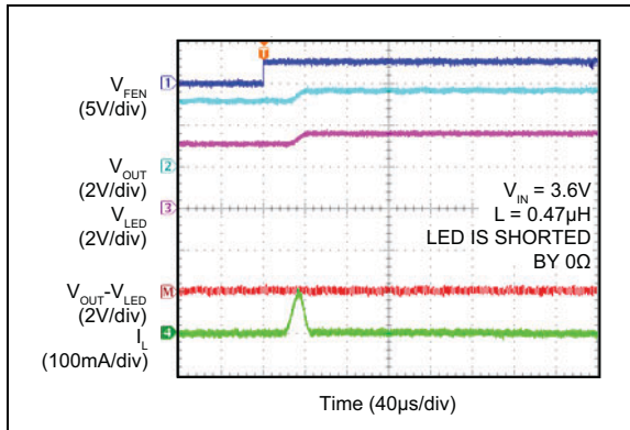
FIGURE 2-19: LED Short-Circuit Protection (LED is Shorted by 0Ω).
