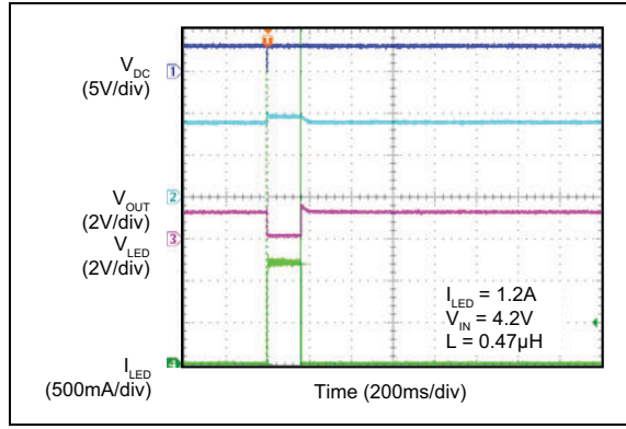
FIGURE 2-18: Flash Safety Timer at 156 ms.
