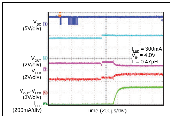
FIGURE 2-16: Torch Mode Turn-On Sequence (Linear Mode).
