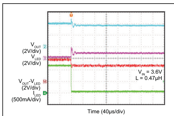
FIGURE 2-26: Load Transient (Flash 1.2A to Torch 63 mA).
