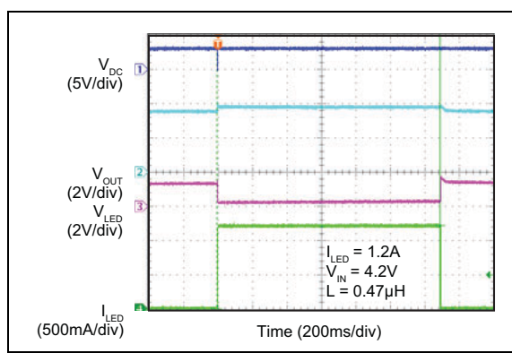
FIGURE 2-17: Flash Safety Timer at 1250 ms.
