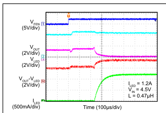
FIGURE 2-14: Flash Mode Turn-On Sequence (Linear Mode).
