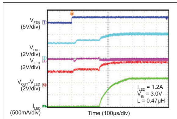
FIGURE 2-13: Flash Mode Turn-On Sequence (Boost Mode).
