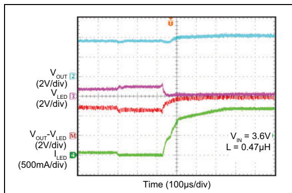
FIGURE 2-25: Load Transient (Torch 63 mA to Flash 1.2A).
