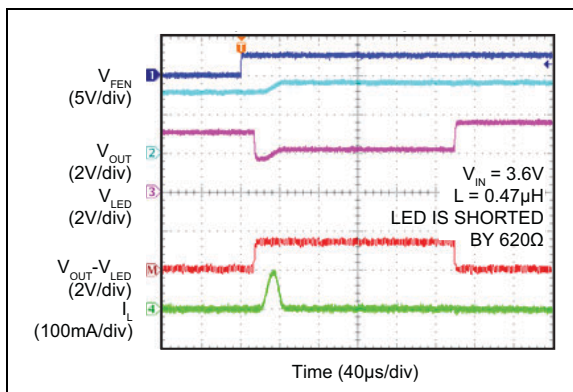
FIGURE 2-20: LED Short-Circuit Protection (LED is Shorted by 620Ω).
