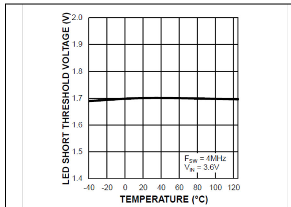
FIGURE 2-6: LED Short Threshold Voltage vs. Temperature.
