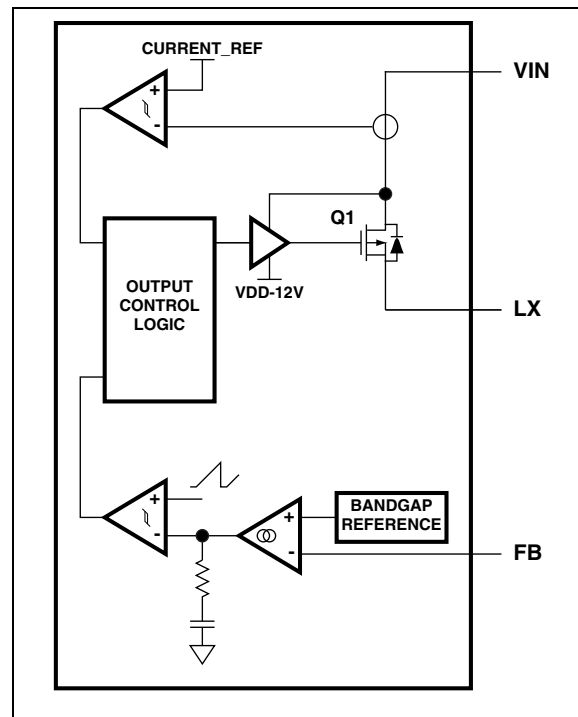
FIGURE 4-2: SMPS Functional Block Diagram.
