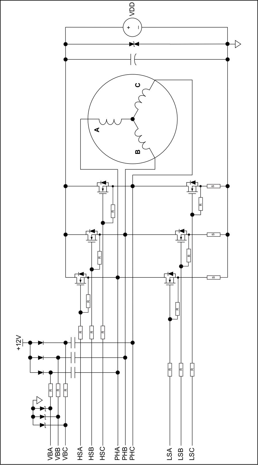
FIGURE 5-3: Overvoltage Protection.
