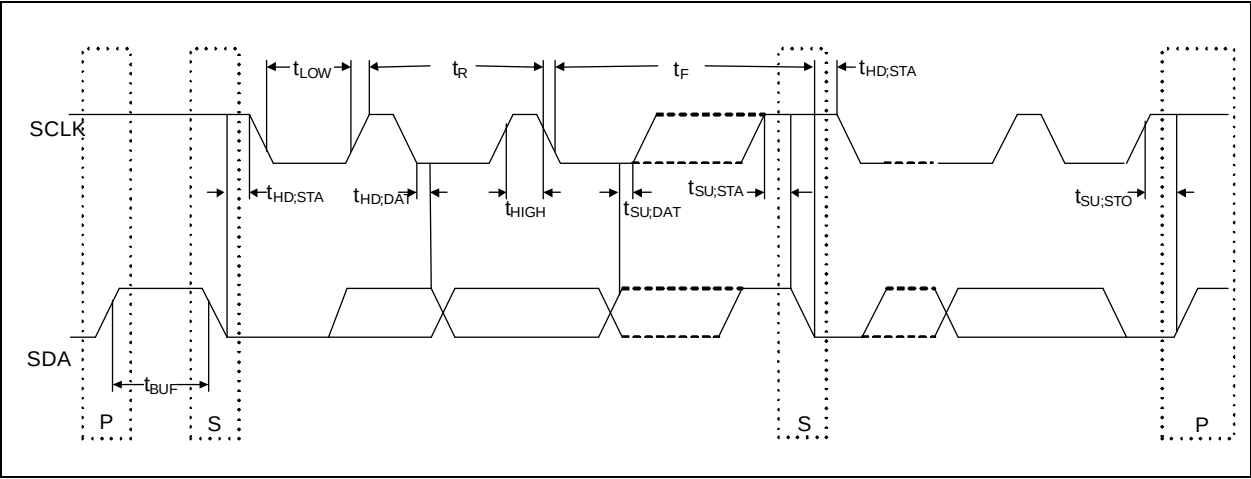
FIGURE 4-2: SMBUS TIMING
