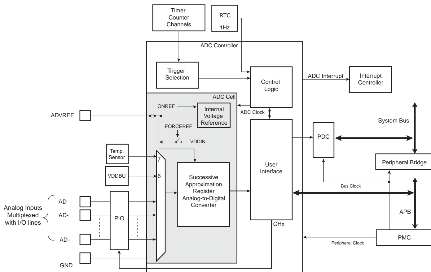
Figure 40-1. Analog-to-Digital Converter Block Diagram
