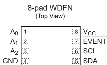
Figure 2-1. Pinout
