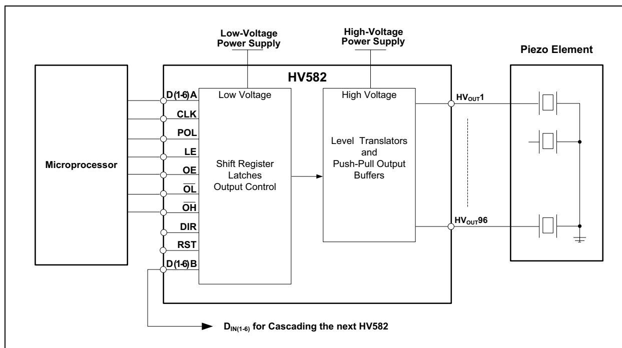
FIGURE 3-1: Typical Application Block Diagram.
