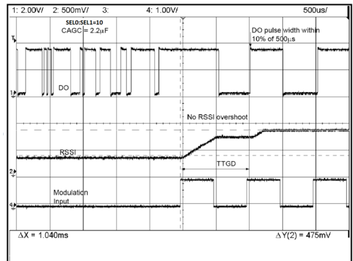
Figure 5. Proper TTGD (1ms) with Sufficient AGC
