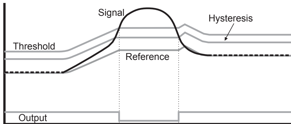
Figure 3-1. Drift Compensation
