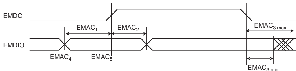
Figure 46-21. Min and Max access time of EMAC output signals
