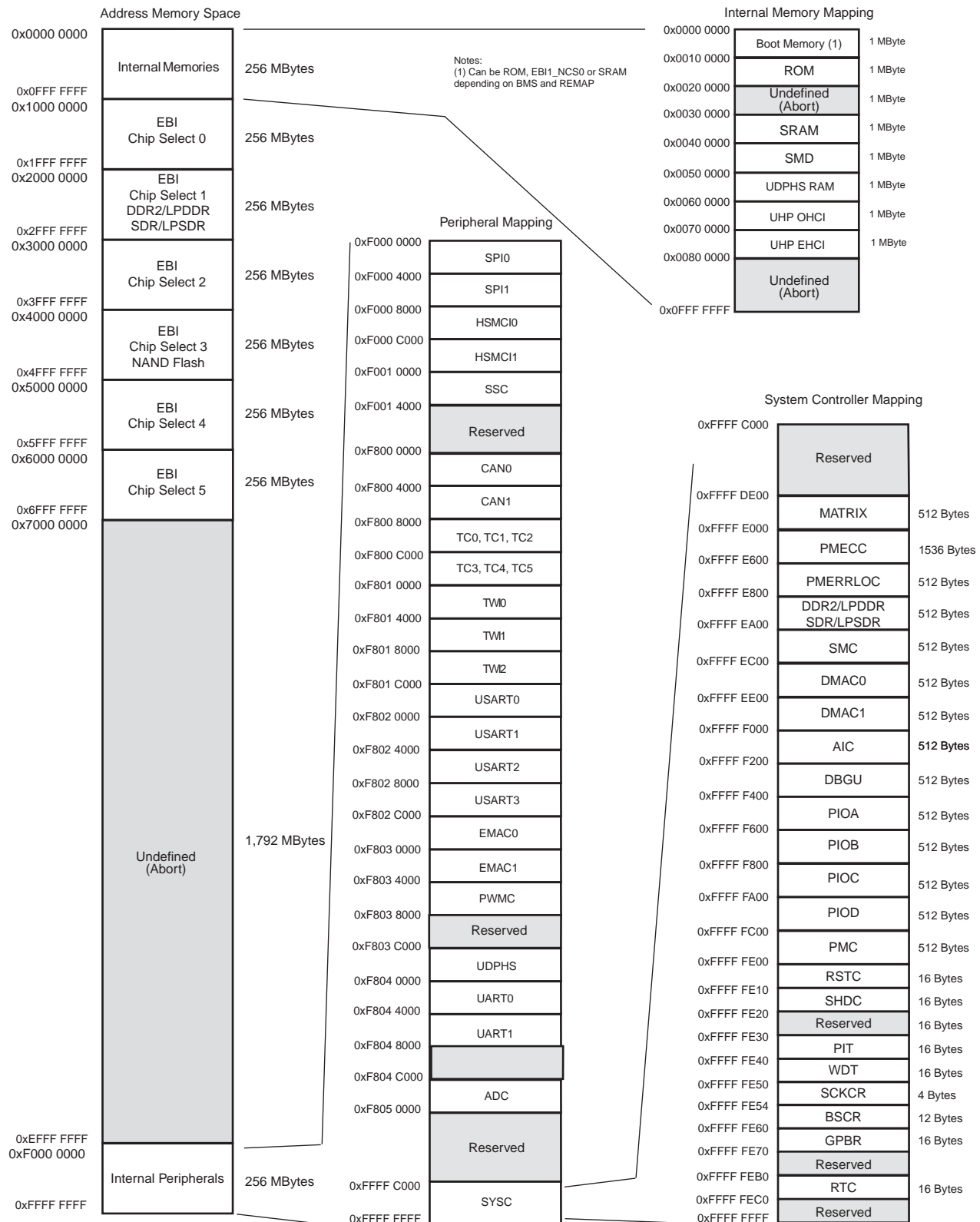
Figure 6-1. SAM9X25 Memory Mapping
