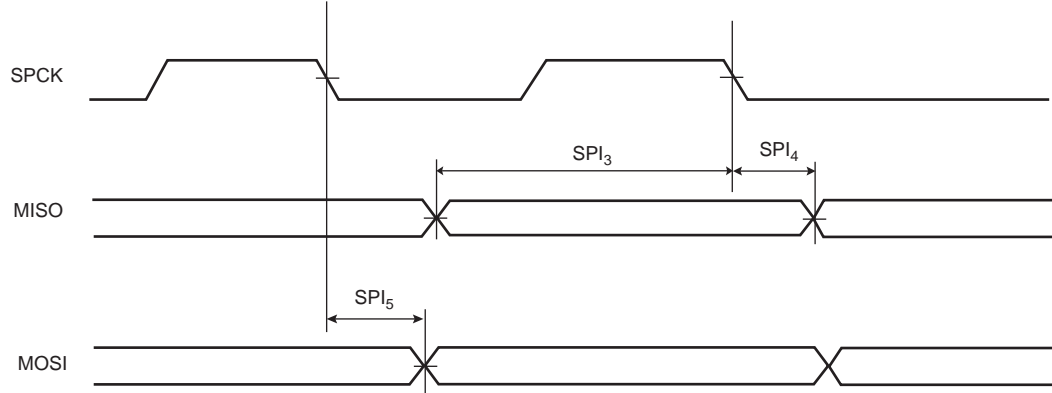
Figure 46-7. SPI Master mode 0 and 3
