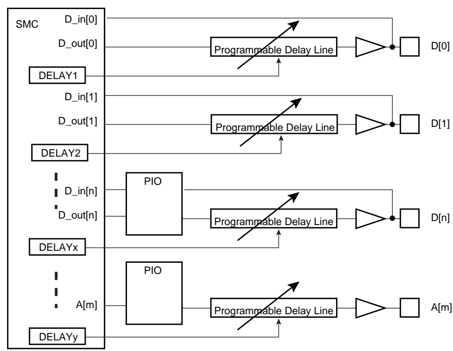
Figure 29-36.Programmable IO Delays
