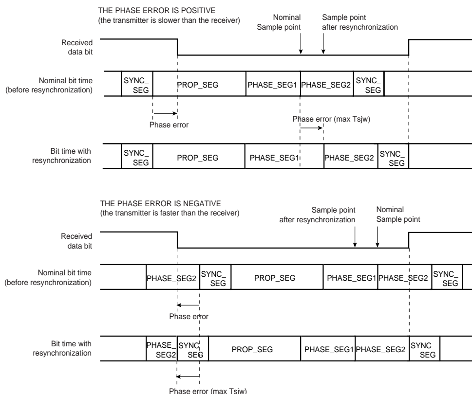
Figure 41-6. CAN Resynchronization
