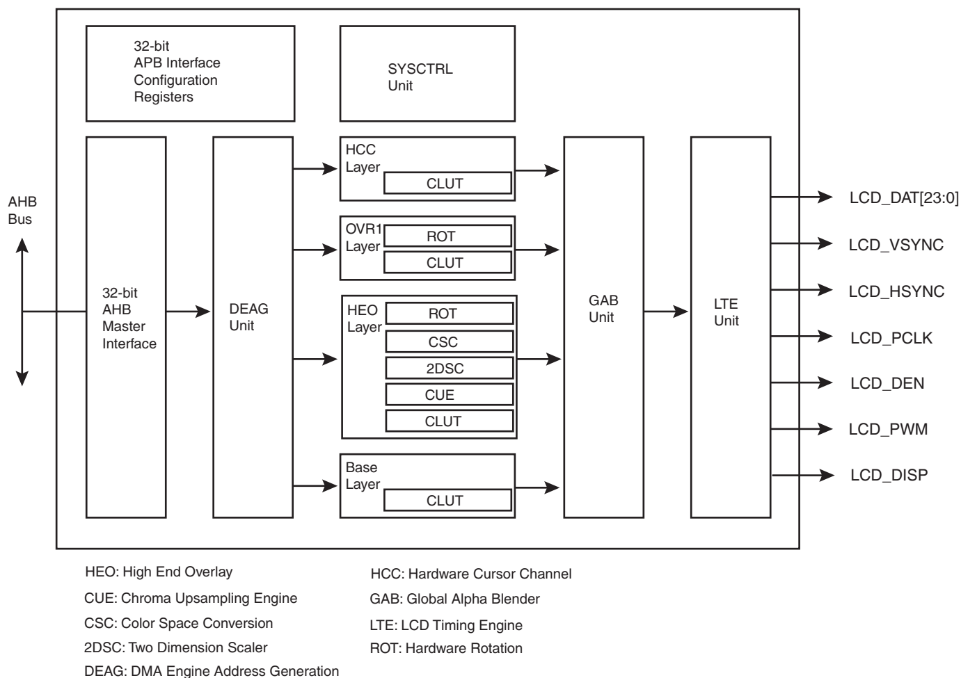
Figure 44-1. Block Diagram
