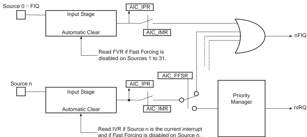
Figure 13-10. Fast Forcing
