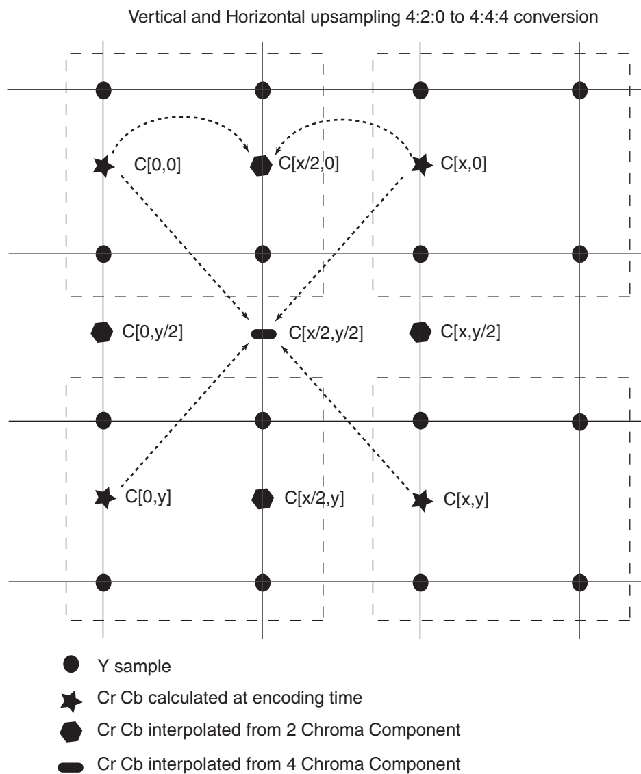
Figure 44-5. 4:2:0 Upsampling Algorithm
