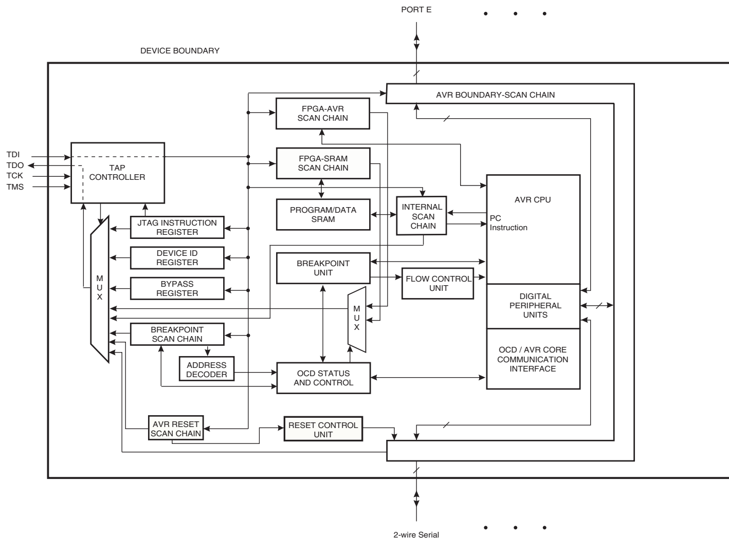
Figure 4-16. Block Diagram
