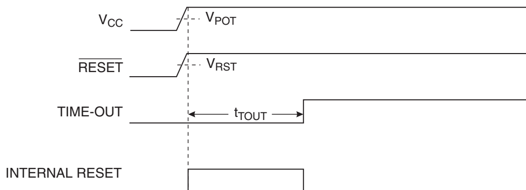
Figure 4-13. MCU Start-up, \overline{RESET} Tied to V_{CC}
