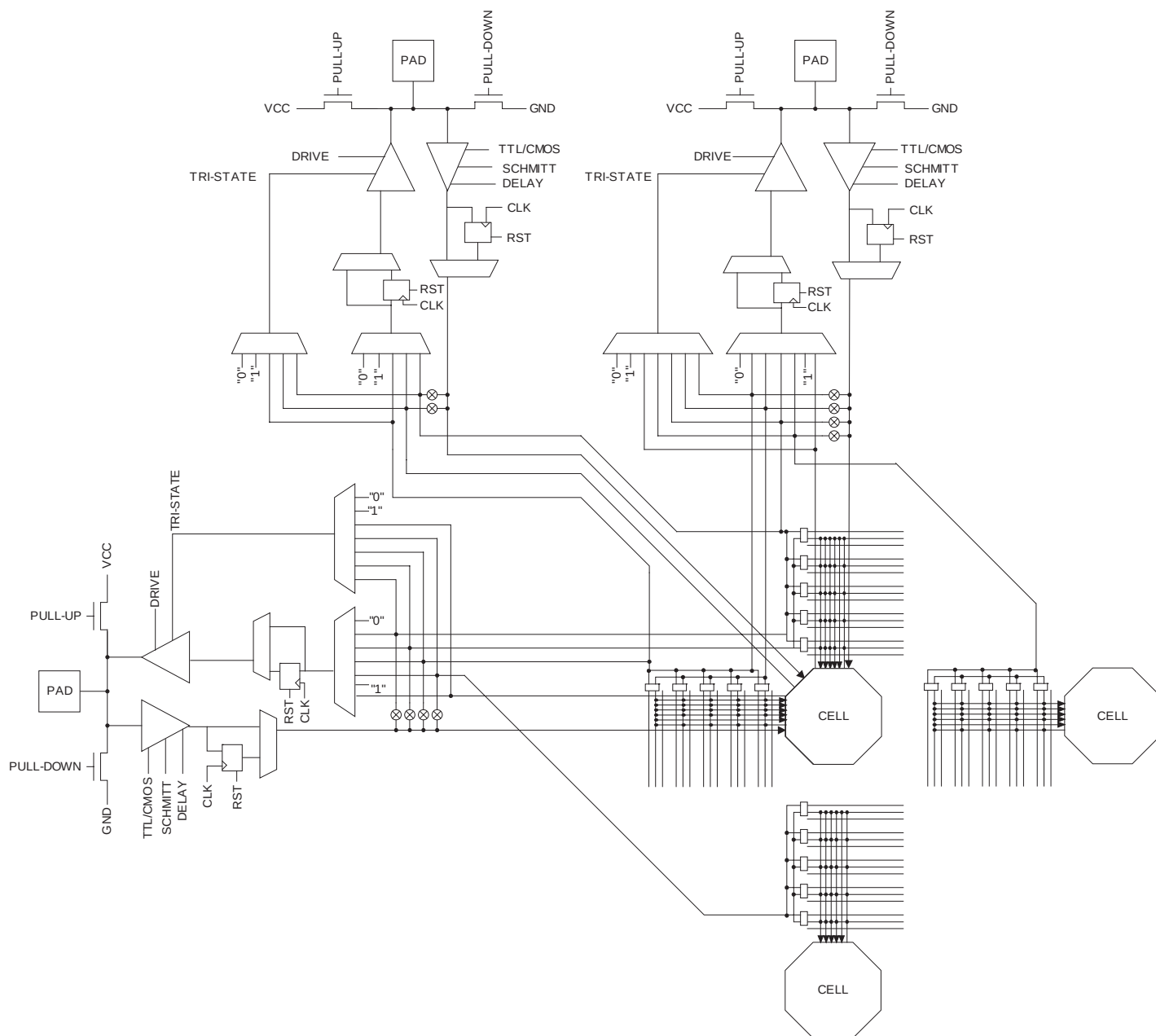
Figure 2-15. Corner I/Os
