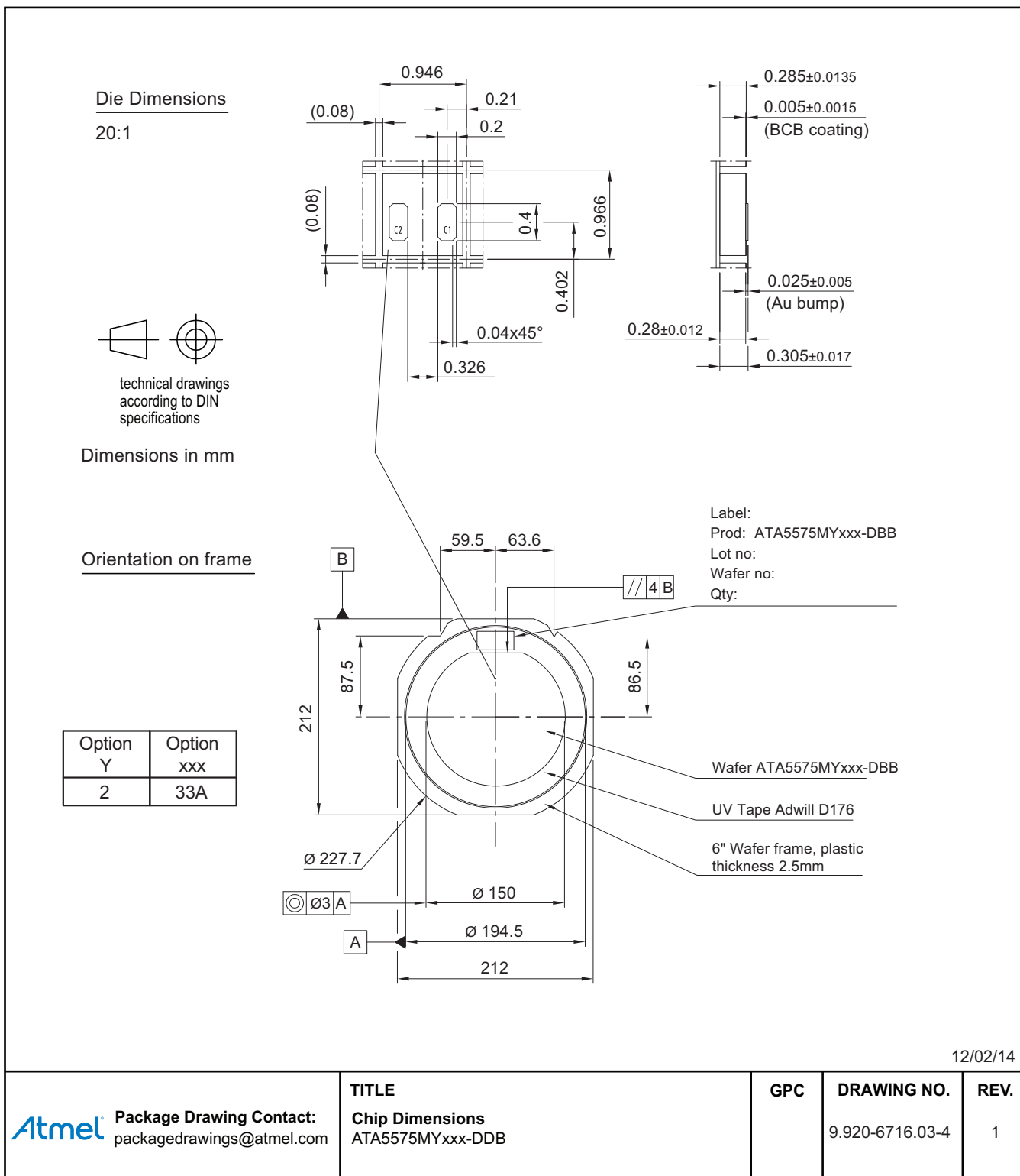
Figure 11-4. 6" Sawn Wafer on Foil 25µm
