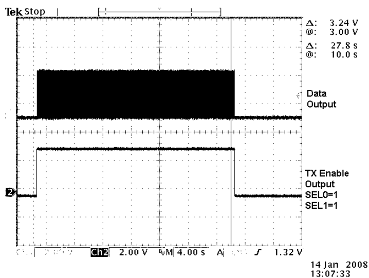
Figure 9. MICRF302 Time
