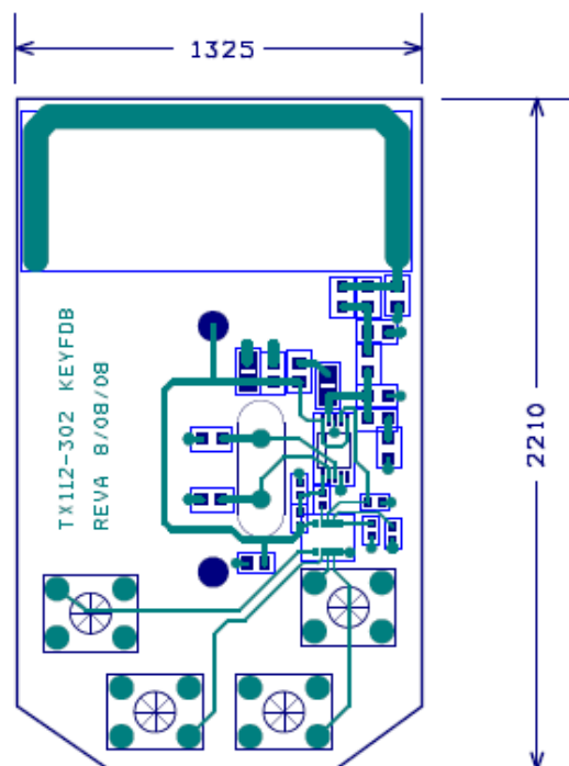
Figure 15. TX112-MICRF302 KEYFOB Evaluation Board, Top View
