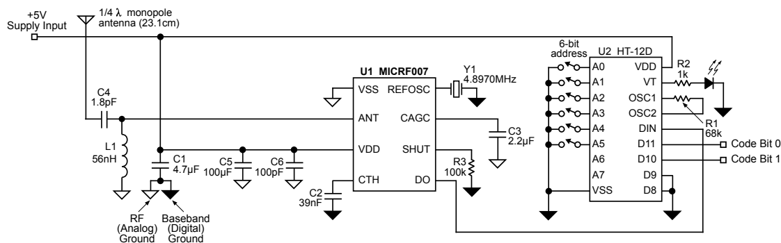
Figure 10. 315MHz, 1Kbps On-Off Keved Receiver with Decoder
