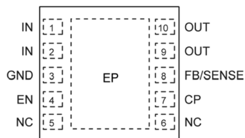
10-Pin 3mm x 3mm MLF ® (ML)
