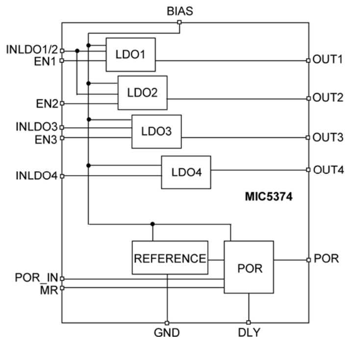
MIC5374 Block Diagram
