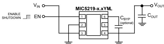
Ultra-Low-Noise Regulator (Fixed)
