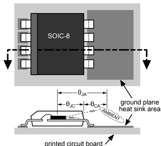
Figure 2. Power SOIC-8 Cross Section
