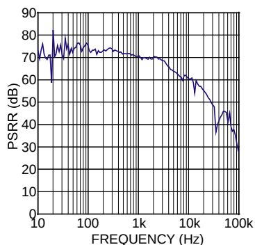
MIC38300 PSRR
