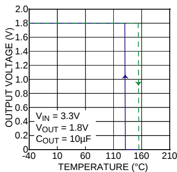
Thermal Shutdown
