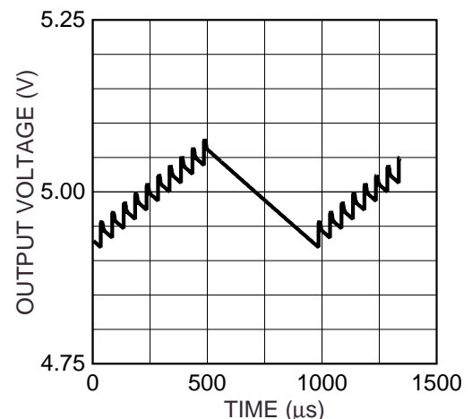
Figure 4. Output Ripple
