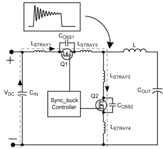
Figure 11. Output Parasitics
