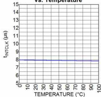
t_{INTCLK} vs. Temperature
