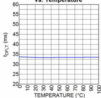
t_{DFLT} vs. Temperature
