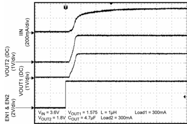
Start-Up Waveform
