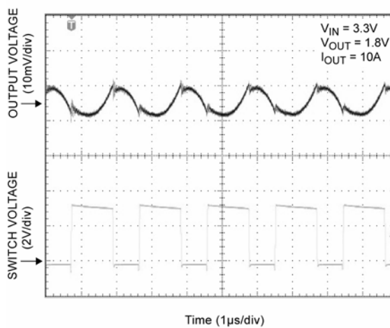
Operating Waveforms
