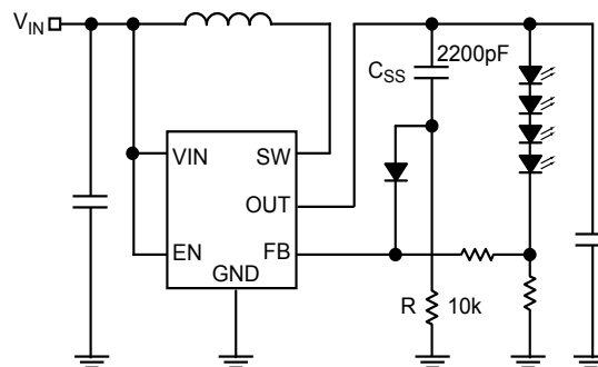
Figure 4. Soft-Start Circuit
