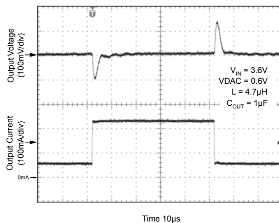
Load Transient
