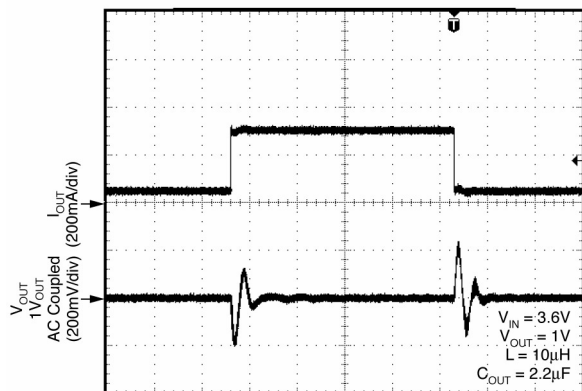
Load Transient
