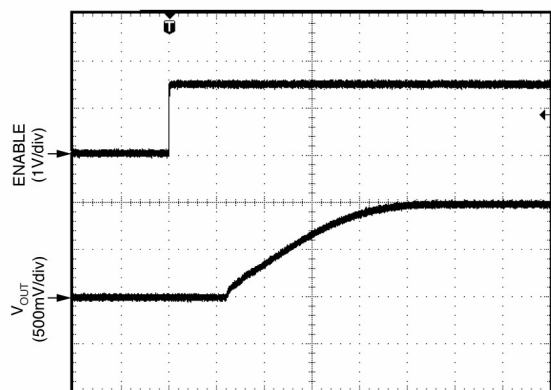
Turn-On Transient
