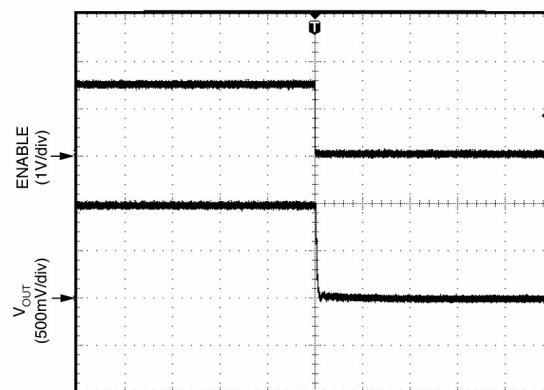
Turn-Off Transient
