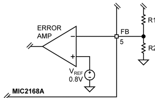
Figure 2. Voltage-Divider Configuration
