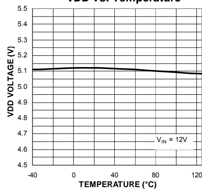
VDD vs. Temperature
