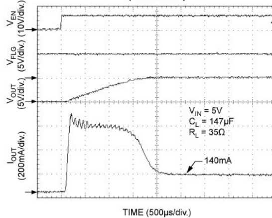
Turn-On (MIC2027-1)
