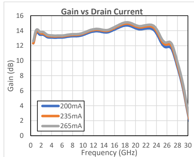
Figure 3 Gain vs I_{DD} ( V_{DD} = 10\text{ V} , T = 25^\circ\text{C} )
