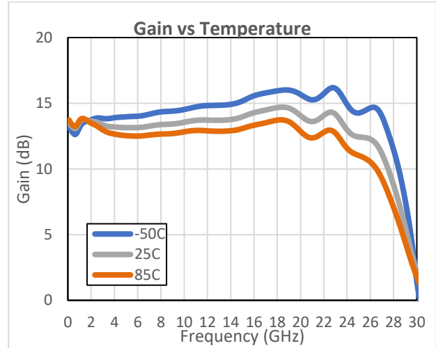
Figure 4 Gain vs Temperature ( V_{DD} = 10\text{ V} , I_{DD} = 235\text{mA} )
