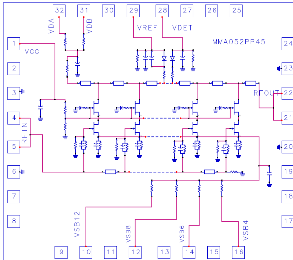
Figure 22 Functional Schematic
