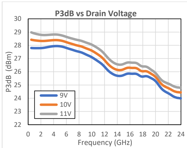
Figure 13 P3dB vs V_{DD} ( I_{DD} = 330\text{mA} , T = 25^\circ\text{C} ) (State 16)
