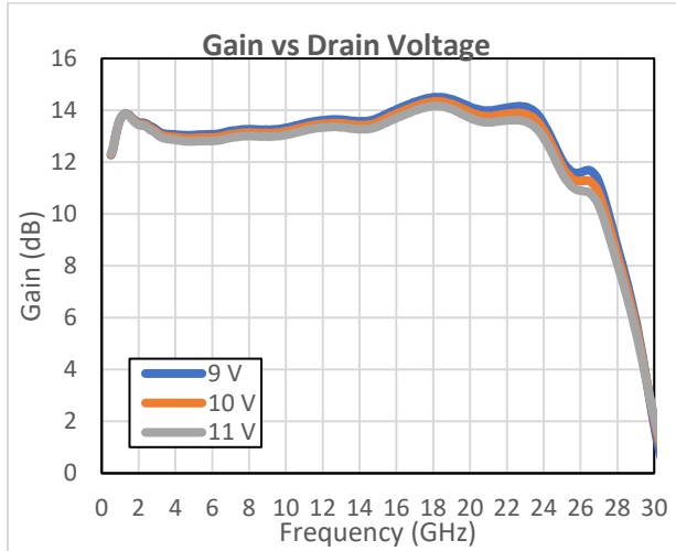
Figure 2 Gain vs V_{DD} ( I_{DD} = 235\text{mA} , T = 25^\circ\text{C} )
