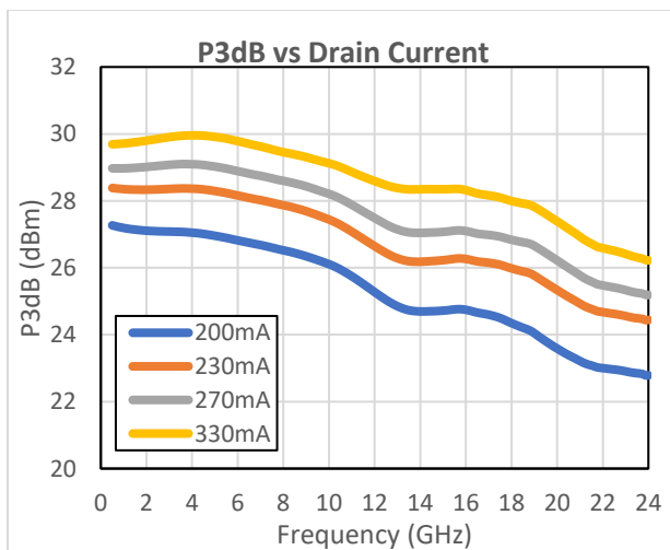
Figure 14 P3dB vs I_{DD} ( V_{DD} = 10\text{ V} , T = 25^\circ\text{C} )
