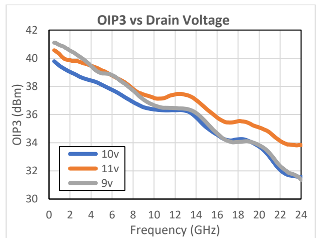
Figure 17 OIP3 vs V_{DD} ( I_{DD} = 235\text{mA} , T = 25^\circ\text{C} , P_{out} = 10\text{dBm} )
