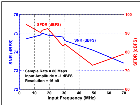
FIGURE 3-31: SNR/SFDR vs. Input Frequency: f_S = 80 \text{ Mps} .
