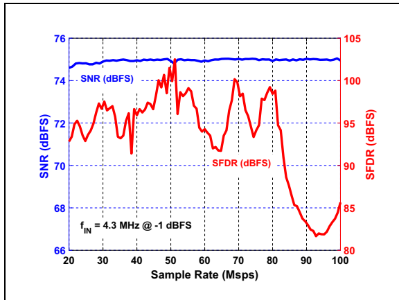
FIGURE 3-30: SNR/SFDR vs. Sample Rate (Mps): f_{IN} = 4.3 \text{ MHz} .
