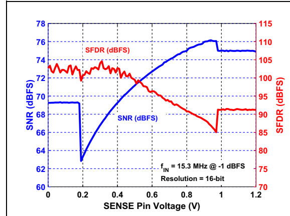
FIGURE 3-32: SNR/SFDR vs. SENSE Pin Voltage: f_{IN} = 15.3 \text{ MHz} .
