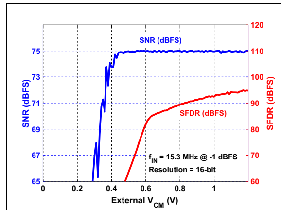
FIGURE 3-34: SNR/SFDR vs. V_{CM} Voltage (Externally Applied): f_S = 80 \text{ Mps} , f_{IN} = 15.3 \text{ MHz} .
