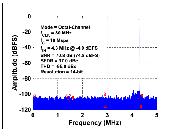
FIGURE 3-22: FFT for 4.3 MHz Input Signal: f_S = 10 Msps, Octal-Ch., A_{IN} = -4 dBFS.
