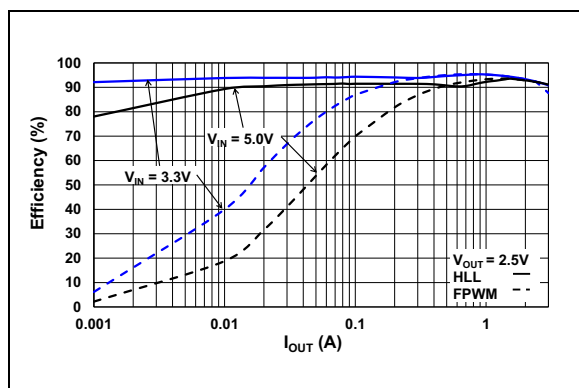
FIGURE 2-8: Efficiency vs. Load Current ( V_{OUT} = 2.5V ).
